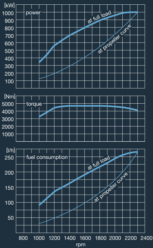
■ V12-1360, 1,000 kW (1,360 mhp)
