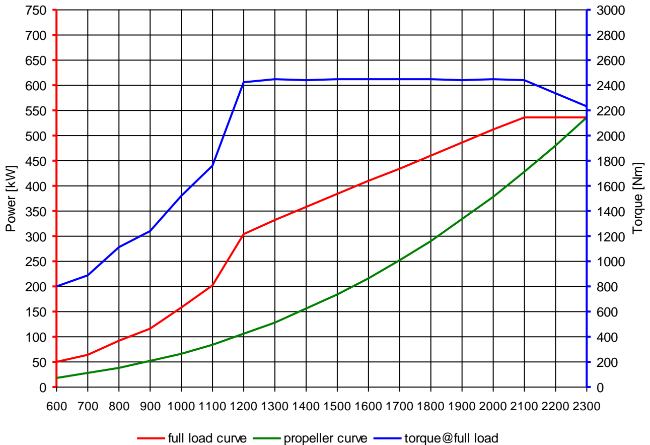
Power/torque curves
