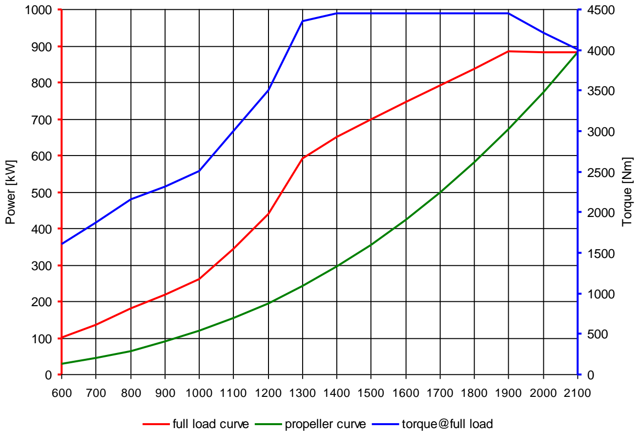
Power/torque curves
