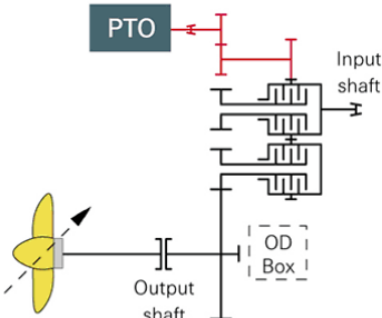
Top PTO73 (R*+NR* Version)
