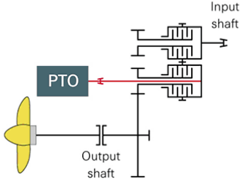
Top PTO71 (R*+NR* Version)
