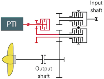
Front PTI24 (R* Version)
