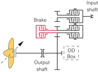
Brake (R* Version)
